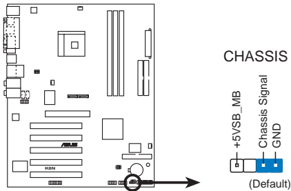
K8N Chassis intrusion connector
