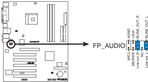
K8N Front panel audio connector
