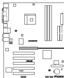
K8N Accelerated Graphics Port (AGP)
