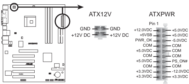
K8N ATX power connectors
