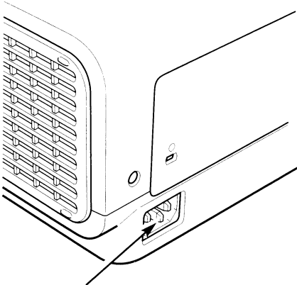
Connect AC power cord (supplied) to the projector. The AC outlet must be near this equipment and must be easily accessible.
