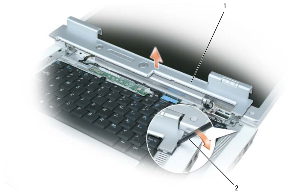
1 铰接护盖
